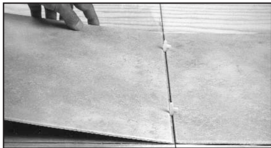
Fig. 14 - Position spacers before setting the tile.
