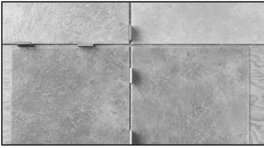
Fig. 21 - Separated border tiles use a spacer one-half the thickness of the whole tiles.
