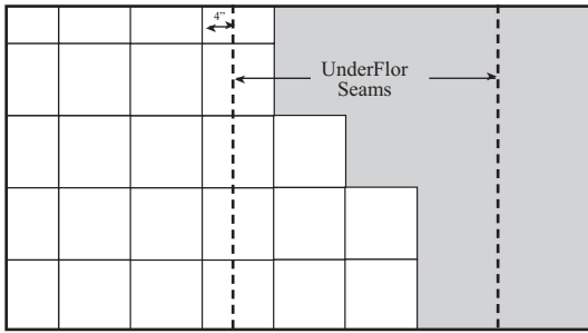
Fig. 6 – Position seams at least 4” away from tile joints.
