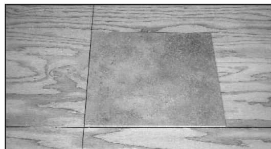
Fig. 11 - Positioning tiles.
