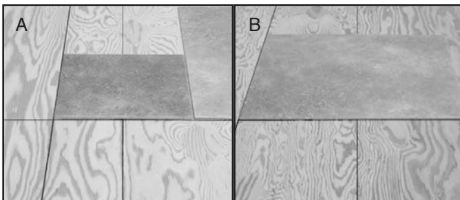
Fig. 24 - Reposition the center lines so the separated tile (A) or the whole tile (B) is at the center of the room to achieve the desired border appearance.
